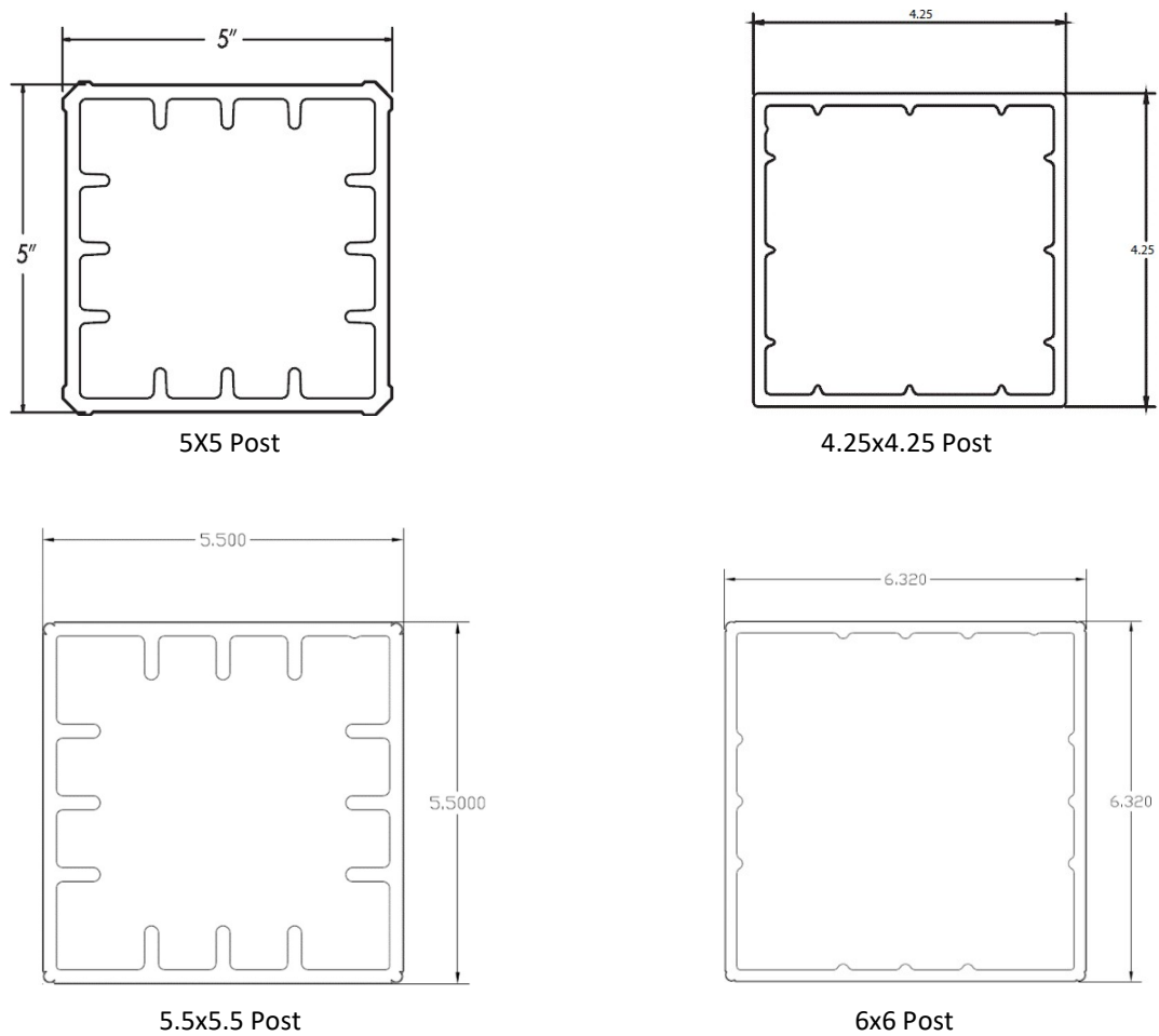
FIGURE 17 - POST SLEEVE PROFILES FOR 4X4 OR 6X6 WOOD POSTS
