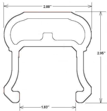
TOP RAIL
