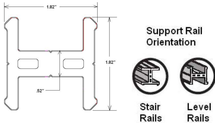
FIGURE 2 – SUPPORT RAIL
