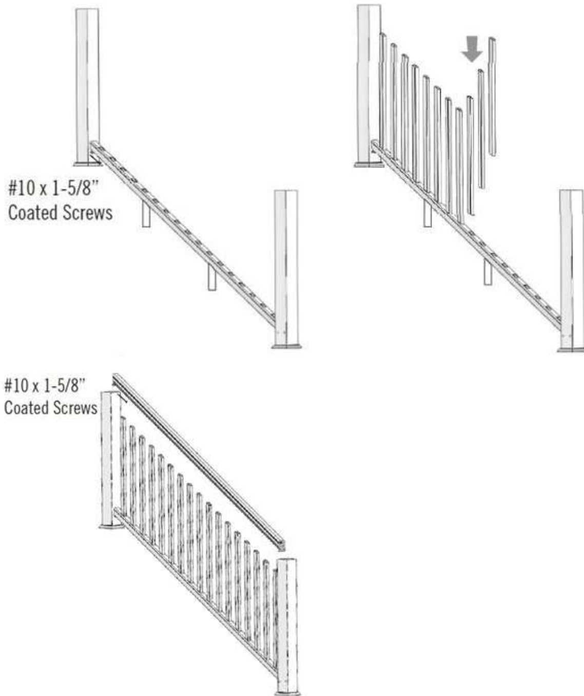
FIGURE 24 - RADIANCERAIL® EXPRESS TYPICAL STAIR ASSEMBLY
