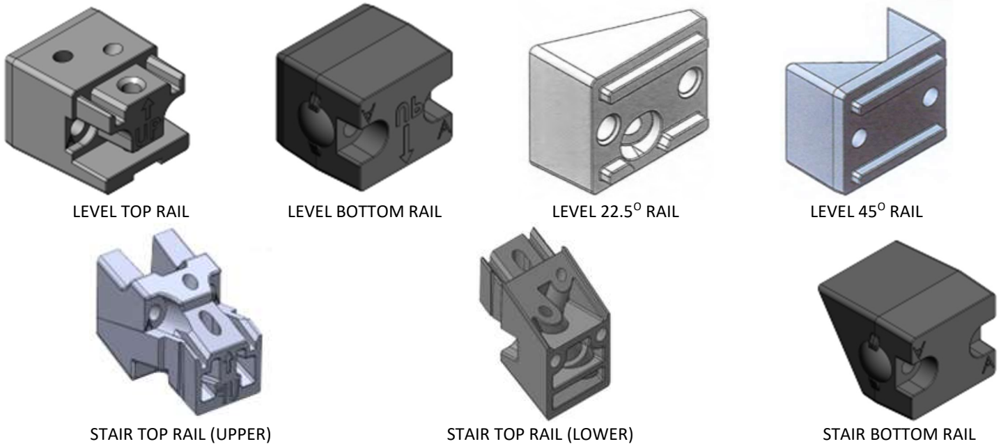
FIGURE 14 – ADVANTAGE RAIL™ BRACKETS
