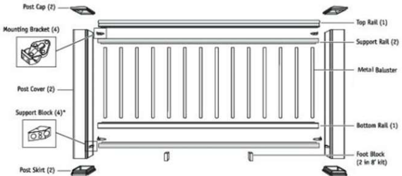
FIGURE 21 – TIMBERTECH® CLASSIC COMPOSITE SERIES AND RESERVE LEVEL ASSEMBLY WITH ALUMINUM BALUSTERS
