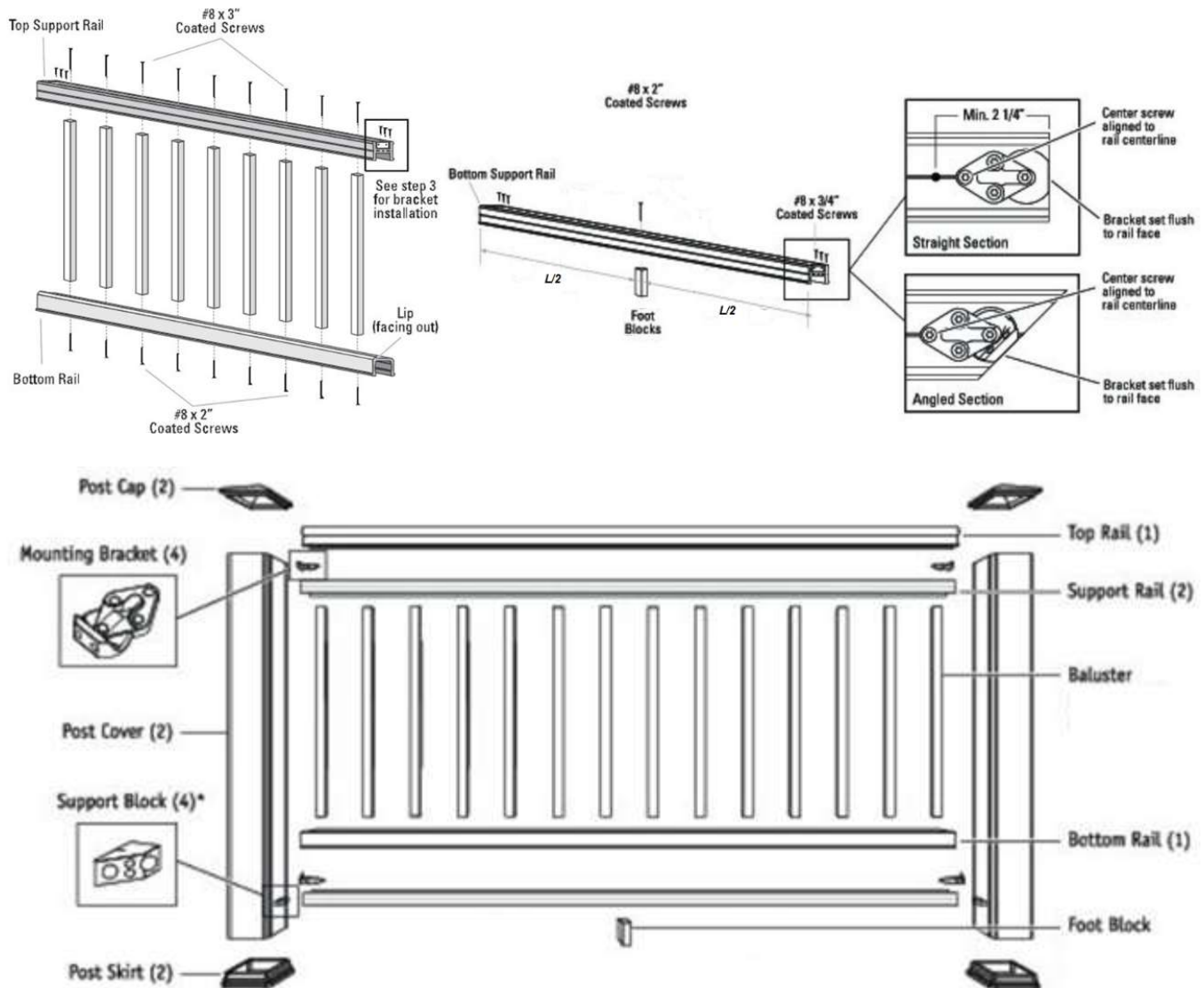
FIGURE 19 – TIMBERTECH® CLASSIC COMPOSITE SERIES AND RESERVE RAIL Level Assembly with Expanded Cellular PVC Balusters
