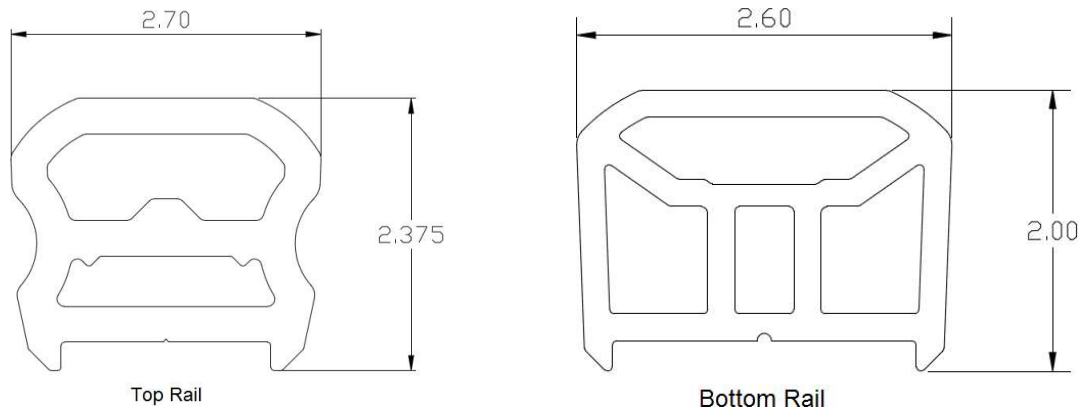
FIGURE 6 - RADIANCERAIL® EXPRESS, RAIL PROFILES
