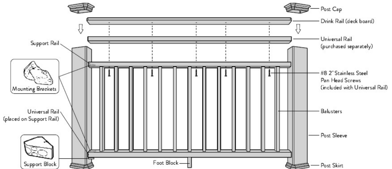
FIGURE 25 – TIMBERTECH® CLASSIC COMPOSITE SERIES DRINK RAIL / CONTEMPORARY RAIL TYPICAL ASSEMBLY Drink Rail / Contemporary Rail may be installed in an over the post configuration.
