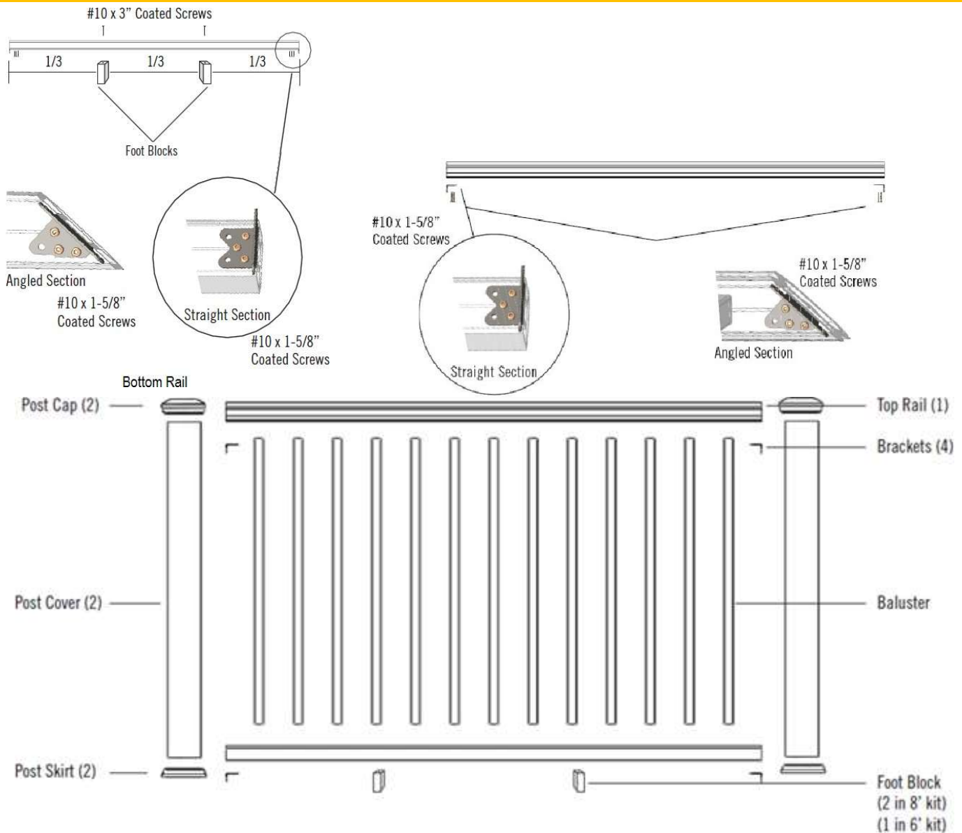
FIGURE 23 - RADIANCE RAIL® EXPRESS TYPICAL LEVEL ASSEMBLY
