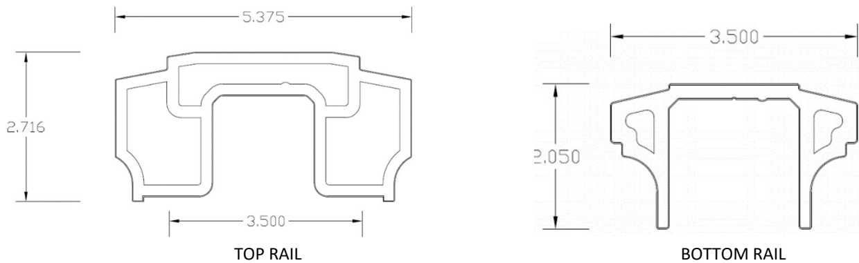
FIGURE 9 – RESERVE RAIL PROFILES
