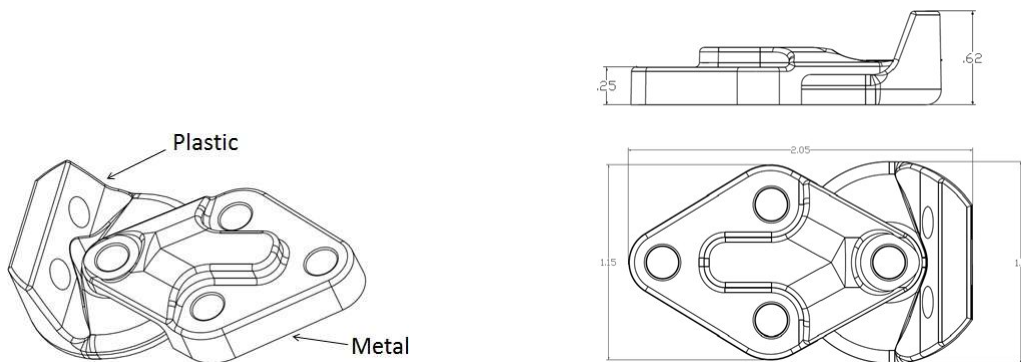
FIGURE 15 – FOUR-HOLE BRACKET TimberTech® Classic Composite Series, Reserve Rail
