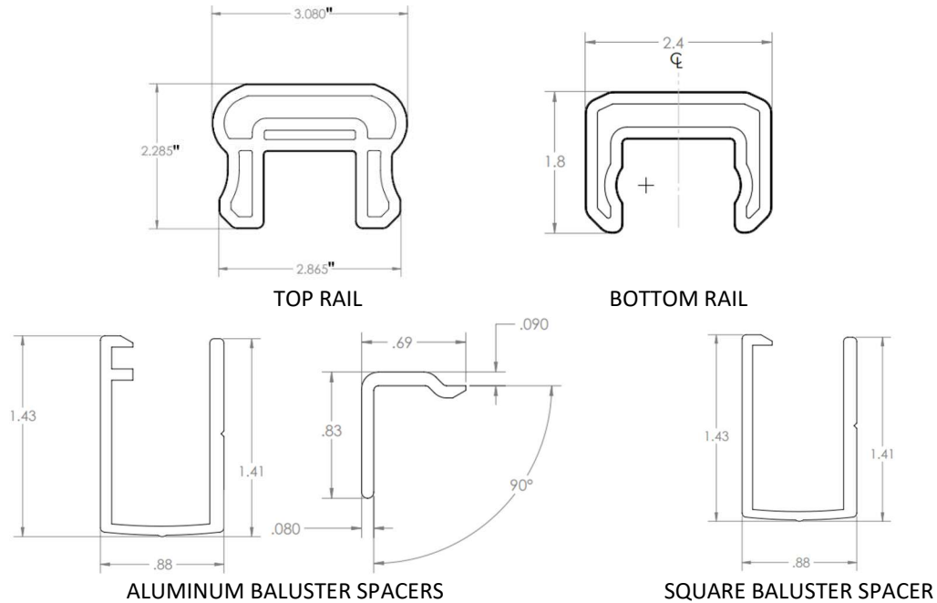
FIGURE 1 – ADVANTAGE RAIL™
