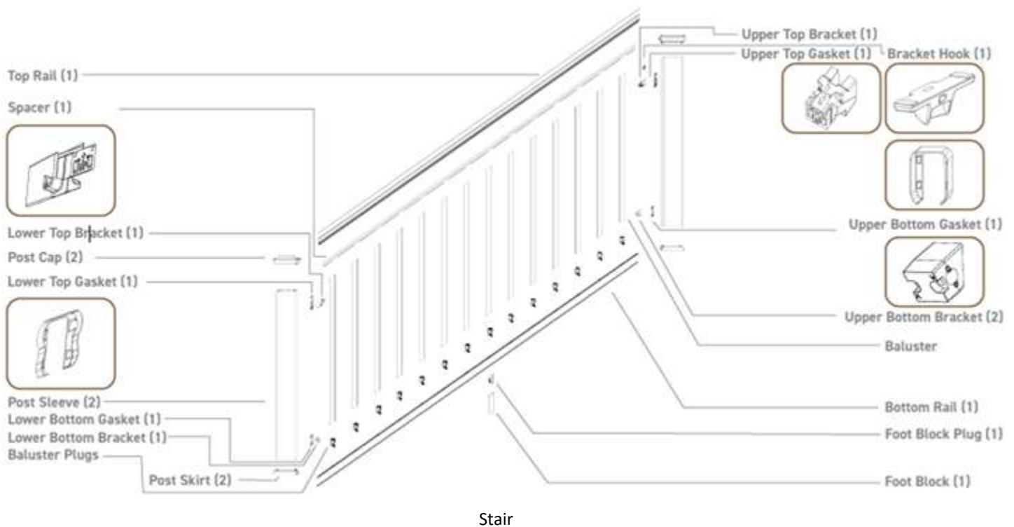
FIGURE 18 – TIMBERTECH® ADVANTAGE RAIL™
