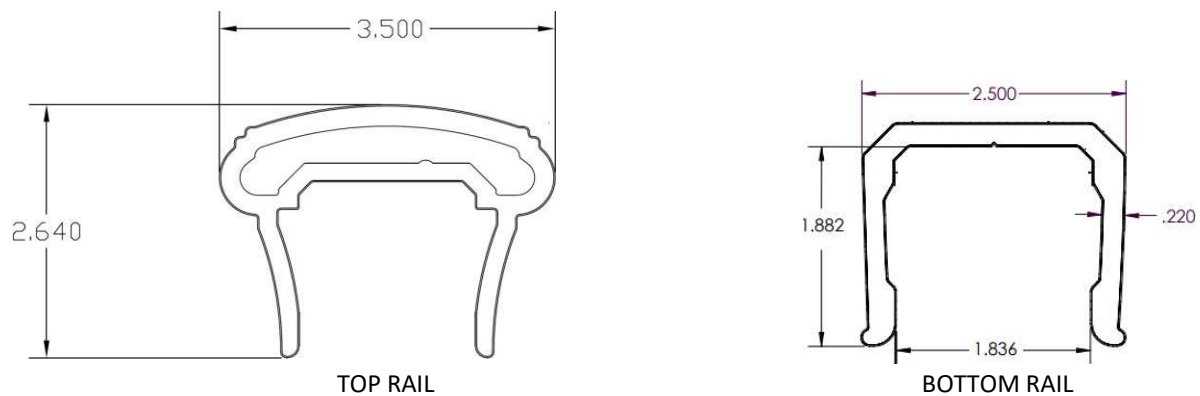
FIGURE 8 – CLASSIC COMPOSITE SERIES TRADEMARK RAIL PROFILES
