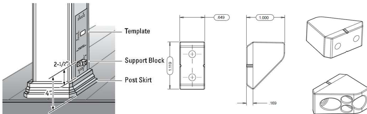
FIGURE 13 - RADIANCERAIL® SUPPORT BLOCK
