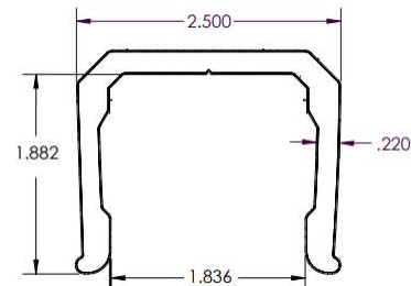
BOTTOM RAIL
