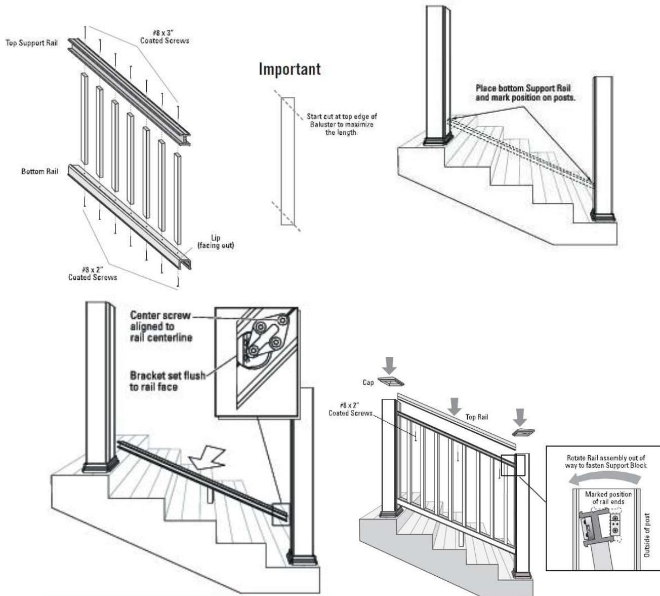
FIGURE 22 - TIMBERTECH® CLASSIC COMPOSITE SERIES AND RESERVE TYPICAL STAIR ASSEMBLY
