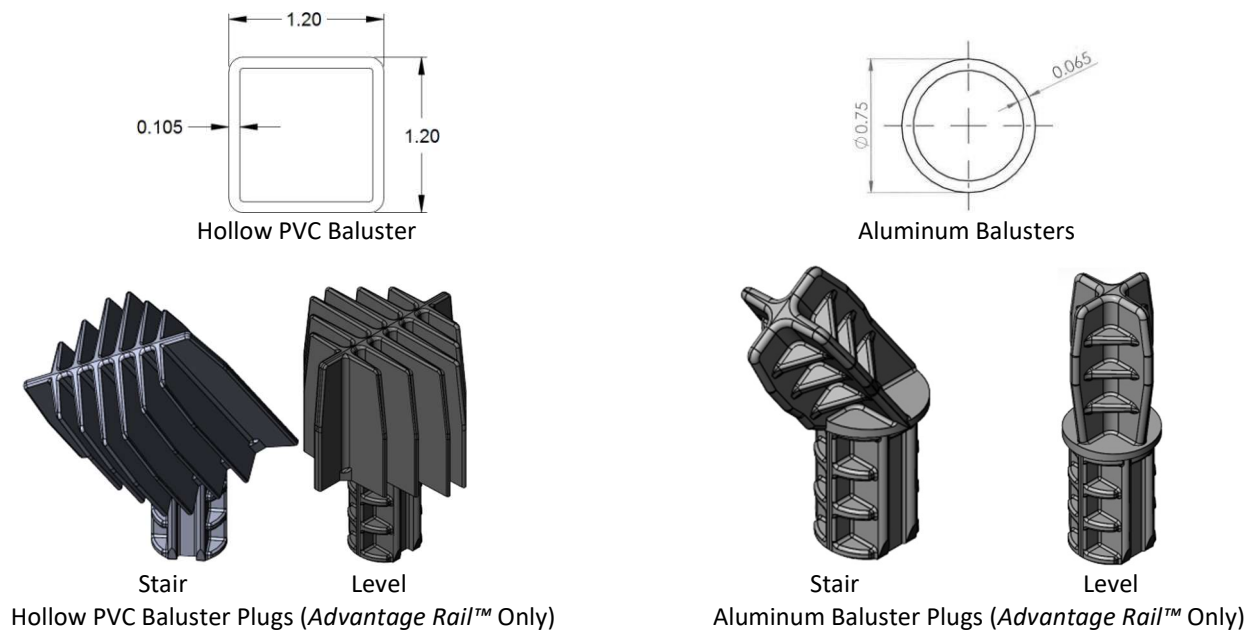
FIGURE 11 – ADVANTAGE RAIL™ AND RADIANCERAIL® EXPRESS BALUSTER PROFILES
