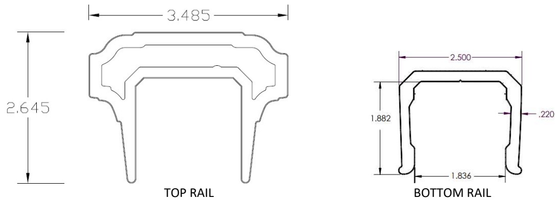
FIGURE 7 – CLASSIC COMPOSITE SERIES PREMIER RAIL PROFILES
