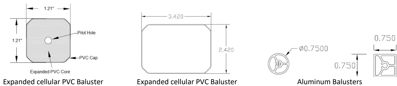
FIGURE 10 - RADIANCERAIL® PREMIER, TRADEMARK, AND RESERVE BALUSTER PROFILES
