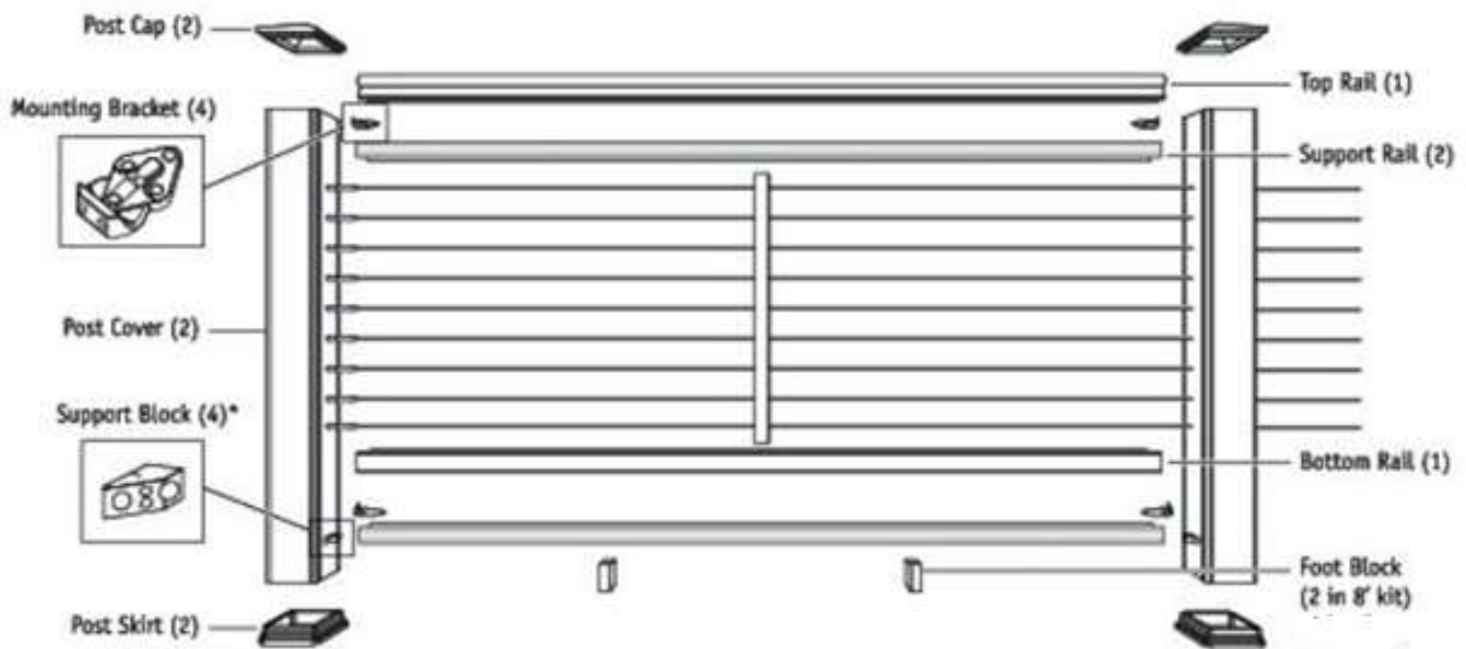
FIGURE 20 – TIMBERTECH® CLASSIC COMPOSITE SERIES AND RESERVE LEVEL ASSEMBLY WITH FEENEY® CABLERAIL™
